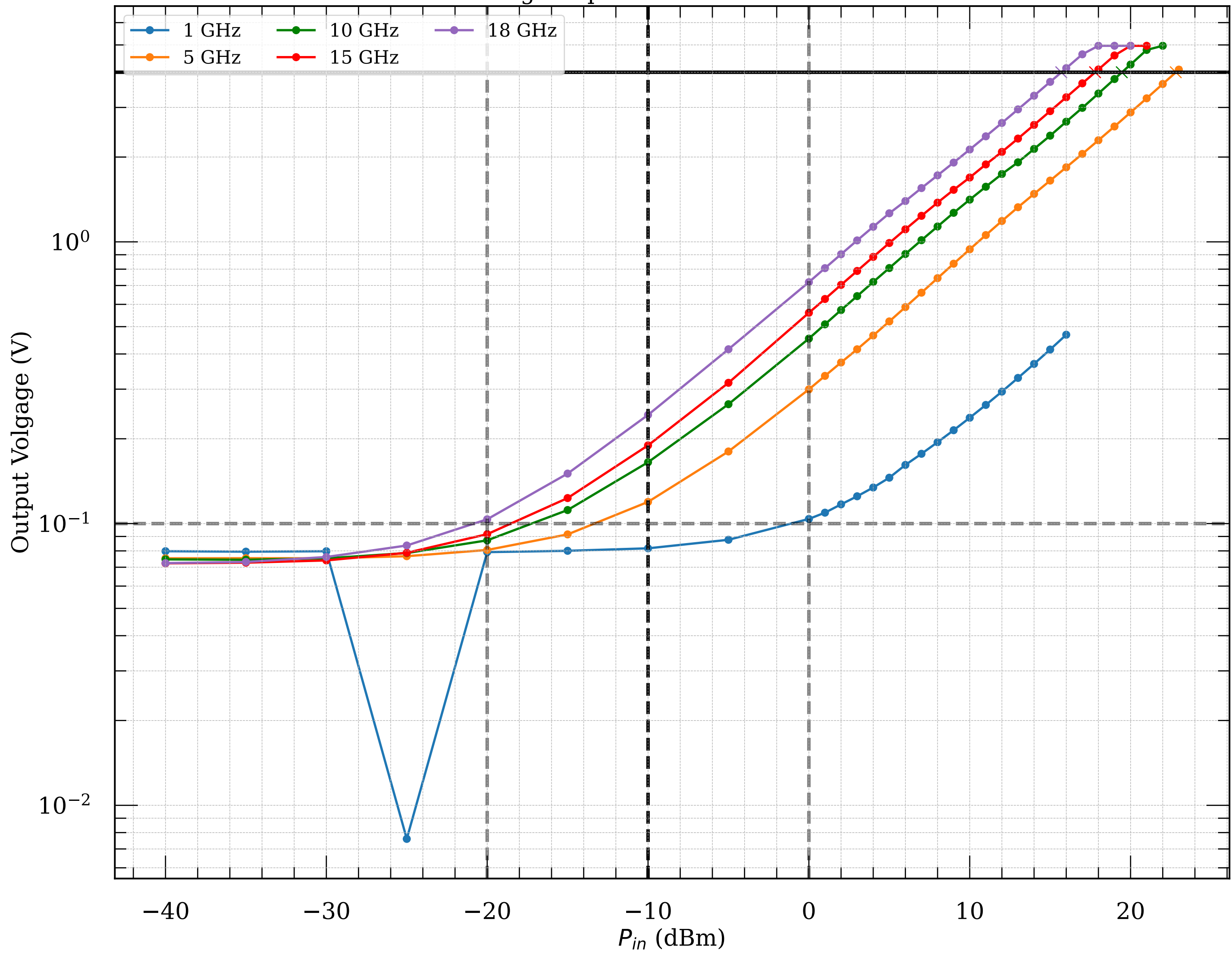
Measured voltage-to-power curve of detector module019
